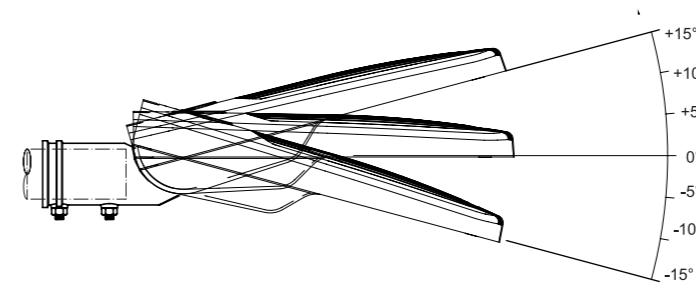
Horizontal Installation
