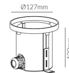
Mounting Sleeve 058
