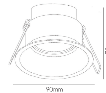
Cutout: Ø75mm
