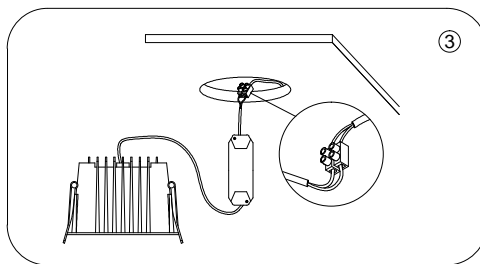
③ Connect AC wire
