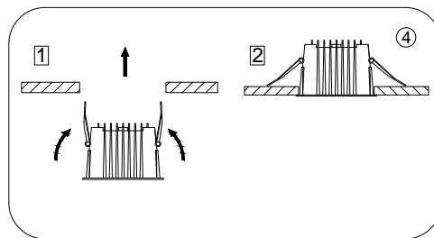
④ Press both side spring clips by hand, push the body of lamp into hole
